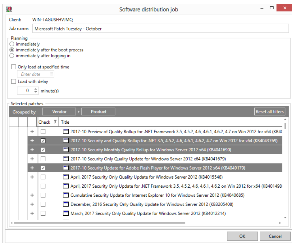
Image 10: G DATA Administrator > Tasks > Software distribution job (Deployment)
