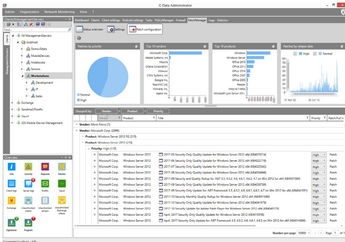
Image 7: G DATA Administrator > PatchManager > Patch configuration
